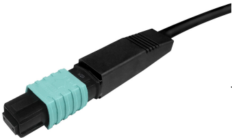
Qwik-Fuse MPO Connector, UNPINNED, OM3/4/5, Aqua, for ribbon, jacketed, 12 pieces pack
