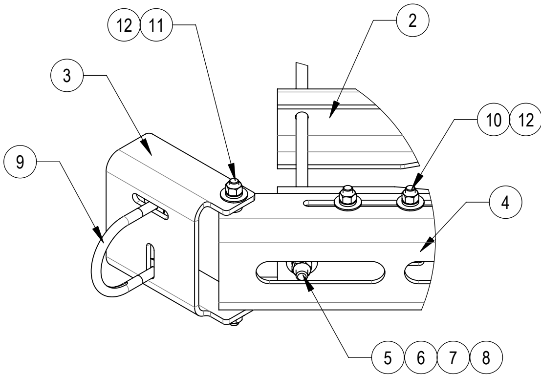
DETAIL B SCALE 1 : 6
