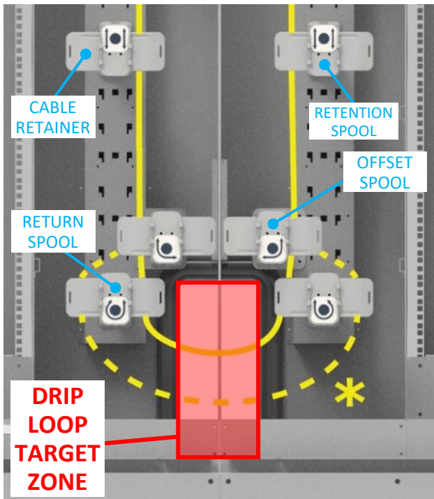
Figure 25. Cable Transition Between Frames
