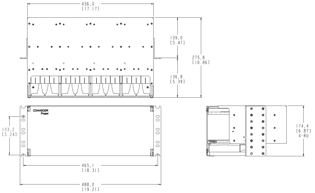
Figure 16. PPL-FA-4U-VCM Panel Dimensions
