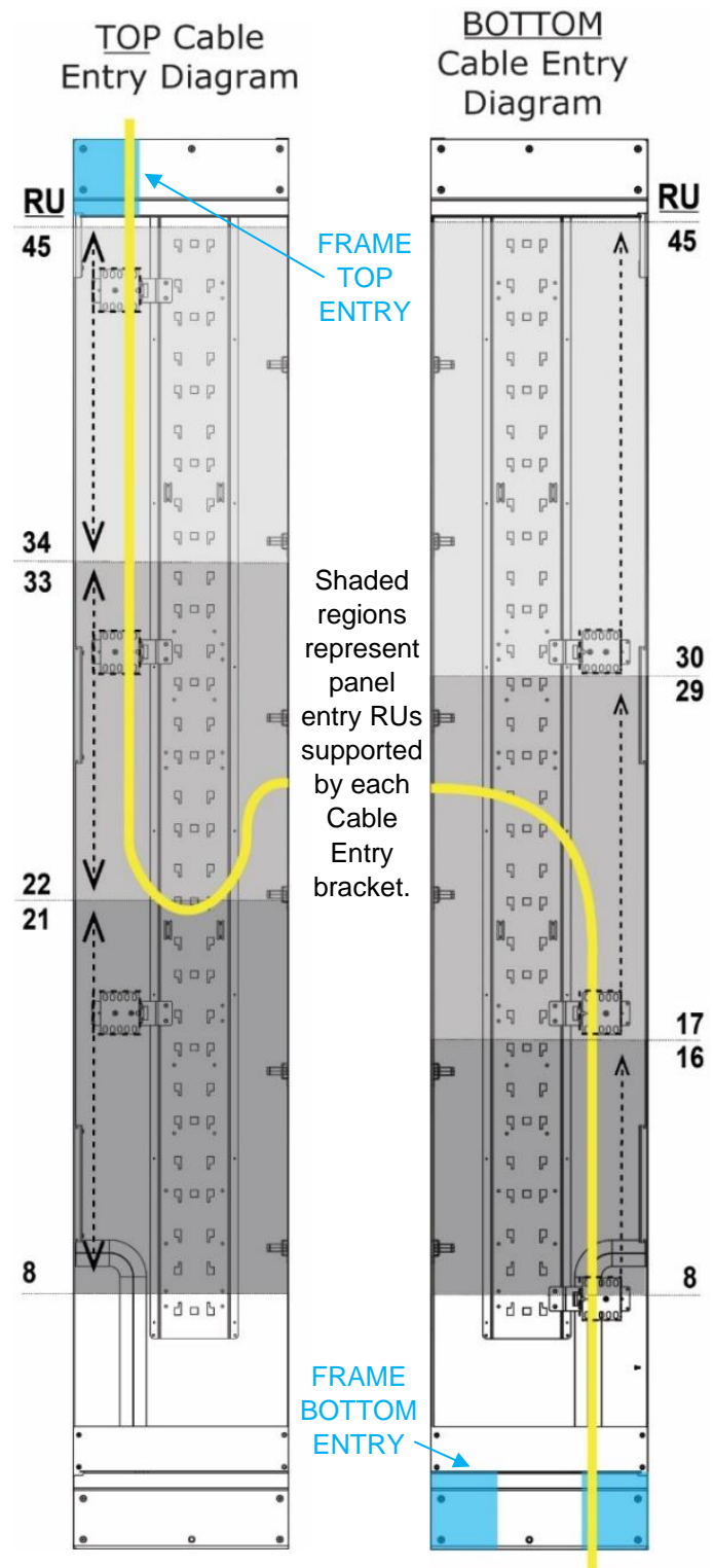
Figure 24. Cable Entry Diagrams
