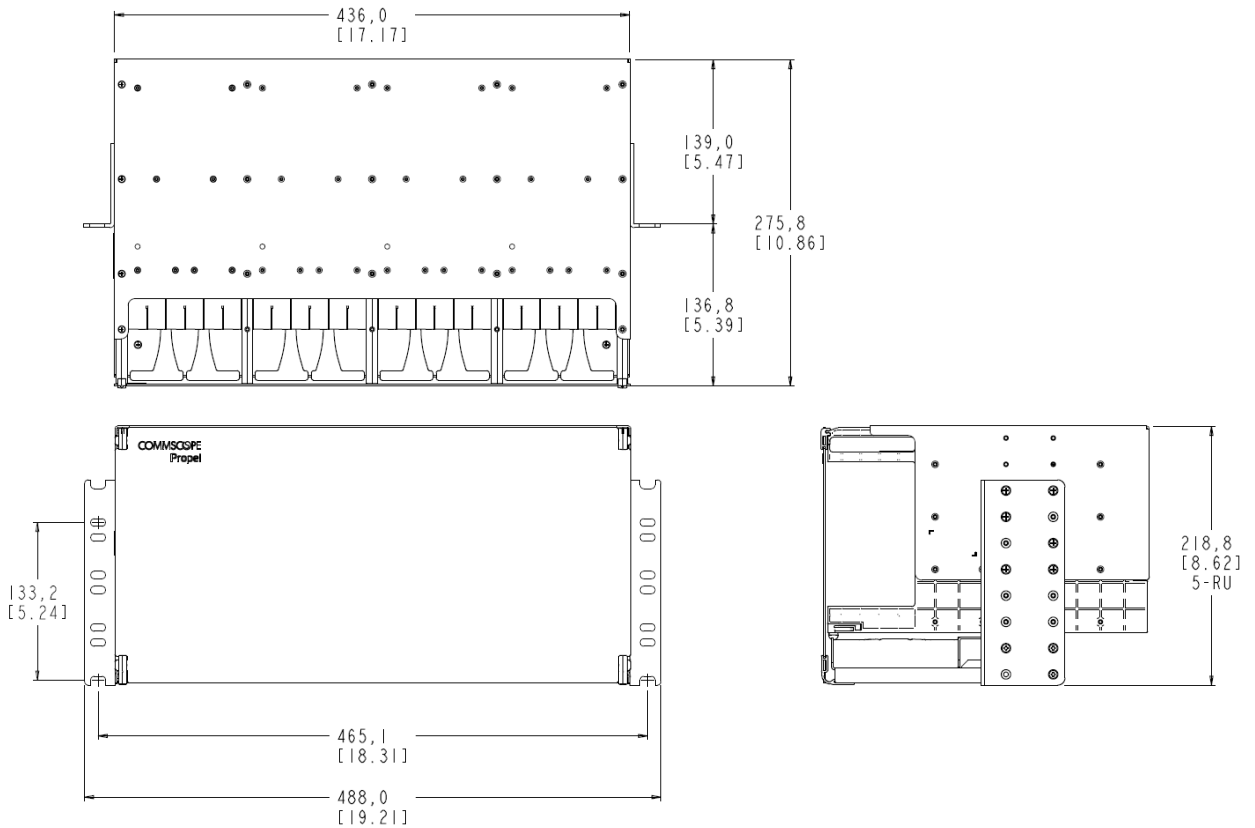
Figure 17. PPL-FA-5U-VCM Panel Dimensions
