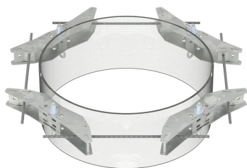
Monopole Hoisting Grip Anchor, for Monopoles 22"-55" OD
