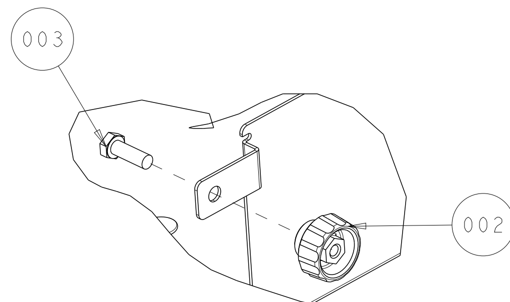
DETAIL C SCALE 5/8
