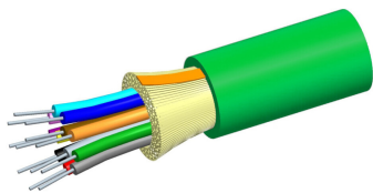
Fiber indoor cable, LazrSPEED® Plenum Distribution Cable, 6 fiber single-unit, Multimode OM3, Feet jacket marking, Green jacket color
