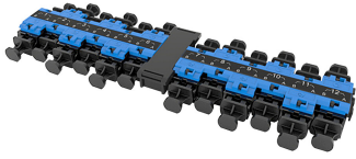
EHD Distribution adapter Pack, Singlemode, 12 LC duplex with dust plugs
