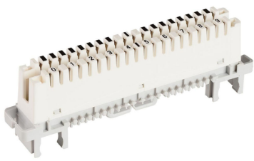
LSA-PLUS® Connection Module, unshielded, 2/10, 10-pair, PROFIL mounting
