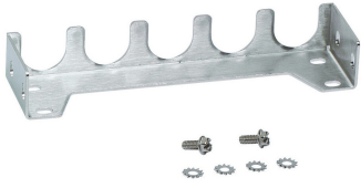
InstaPATCH® Plus Attachment Bracket, Rack Mounted, Five 3/4" fittings
