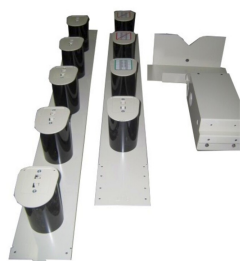
FDF Interbay Management Panel, 7 ft x 5 in x 15 in, 8 in deep troughs /spools, overhead/underfloor
