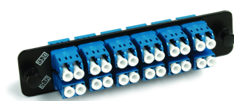
Adapter Pack, Black, 1000-Type, with 12 TeraSPEED® Singlemode duplex LC adapters, blue, no shutter
