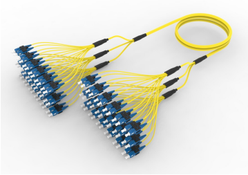
Ultra Low Loss ULL TeraSPEED® SC/UPC to SC/UPC Ruggedized fanout Cable, 36-Fiber, LSZH, 12 fiber PmP 2.0 mm /B2ca
