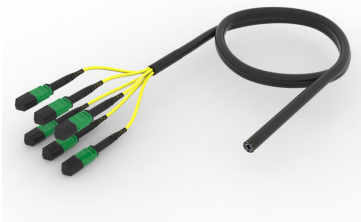
Ultra Low Loss Singlemode MPO12 Pinned to Unconnectorized 72-Fiber Pre-terminated Trunk Cable, Indoor/Outdoor, Low Smoke Zero Halogen /Riser
