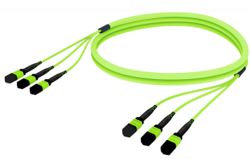
Ultra Low Loss (ULL) OM5 MPO12 (Unpinned) to MPO12 (Pinned), Fiber Trunk Cable Assembly, 36-Fiber, Low Smoke Zero Halogen (LSZH)
