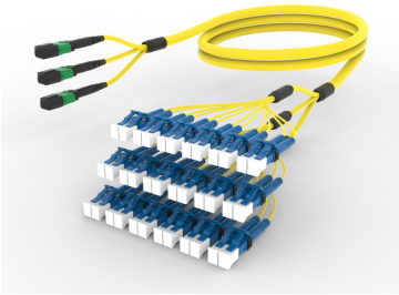
Ultra Low Loss Singlemode, MPO8 (Unpinned) to LC/UPC Uniboot, Fiber Extension Cable Assembly, 24-Fiber, Plenum
