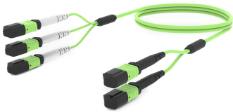
Ultra Low Loss OM5, MPO8 QSFP (Unpinned) to MPO12 (Pinned), Fiber Extension Cable Assembly, 24-Fiber, Plenum
