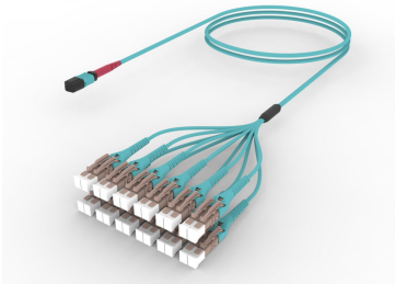
Ultra Low Loss OM4 MPO24 Unpinned to LC/UPC Uniboot 24-Fiber Plenum Array Cord
