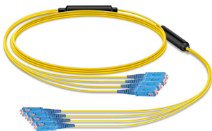
Fiber Optic Patch Cord, OS2, SC/UPC-SC/UPC, 4-fiber RBR, 2.0 mm subunits, 22 m, yellow, 39"/25" breakouts
