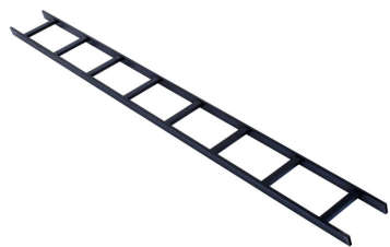
Cable Runway, 6 ft (1829 mm) L x 6 inch (152 mm) W, black
