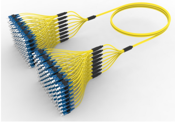
Ultra Low Loss ULL TeraSPEED® SC/UPC to SC/UPC Ruggedized fanout Cable, 96-Fiber, LSZH, 12 fiber PmP 2.0 mm Dca
