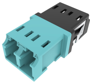
LazrSPEED®, OptiSPEED®, TeraSPEED® LC Duplex Keyed Hybrid Adapter, Aqua/Black, Single Pack
