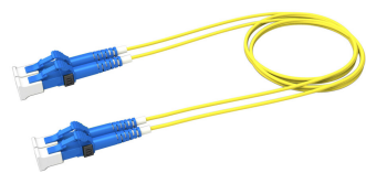
Fiber Optic Patch Cord, Duplex, Singlemode, LC/UPC to LC/UPC, yellow, 2.2 m
