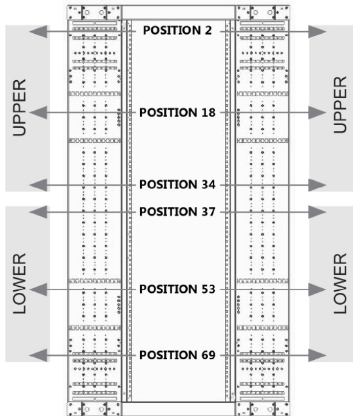
CAGE NUTS POSITIONS FRAME
