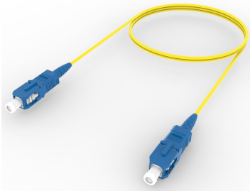
Fiber Optic Patch Cord, singlemode, 1.2 mm OFNP jacket, SC/UPC-SC/UPC, yellow
