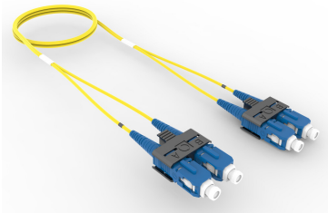
Fiber Optic Patch Cord, duplex, singlemode, 1.2 mm OFNP jacket, SC /UPC-SC/UPC, yellow
