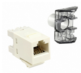
SL110 Series Modular Jack, RJ45, category 6, T568A/T568B, unshielded, without dust cover, light almond
