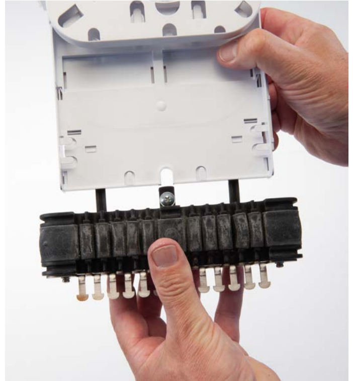
5.2 Install the wedge (if needed).
