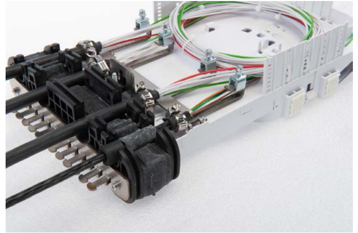
7.1.2 Bracket 1 installed.
