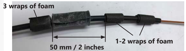
7.2.1 Apply foam tape and 50 mm gel strip.
