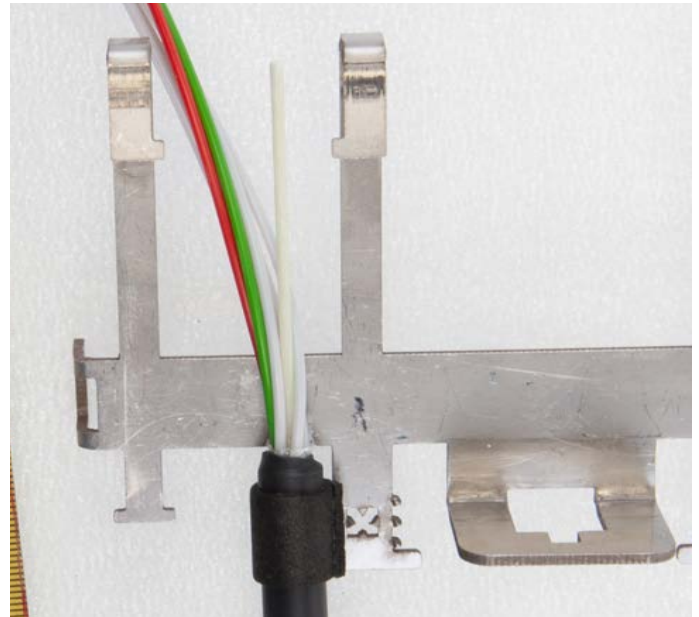
6.1.4 Apply a layer of foam at the jacket end.
