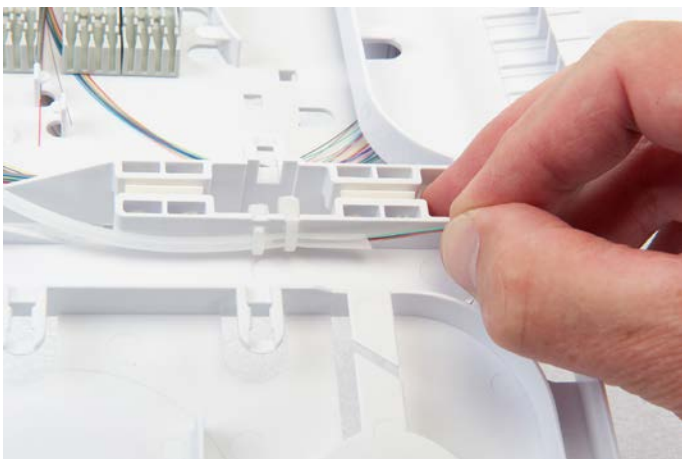
11.3 Install the splitter. Route all fibers through the transportation tube to tray 1 (using a figure of 8 for the feeder fiber to maintain the correct bend radius).
