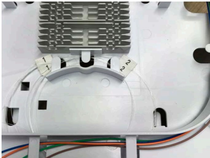
Input fiber labeled number 1. Thru fiber labeled number 2.
