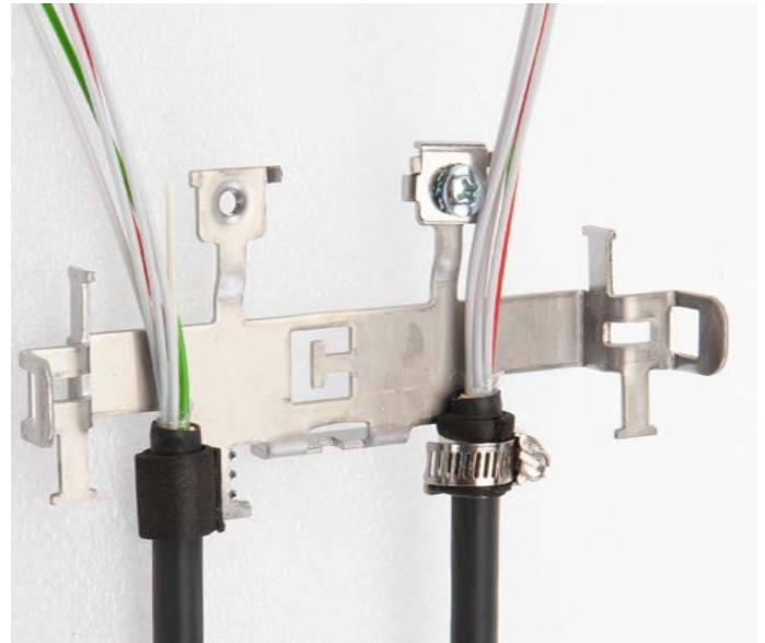
6.2.4 Apply a layer of foam at the jacket end. Secure strength members with metal plate and screw.
