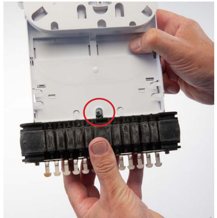
5.3 Slide the gel block on to the organizer. Verify the correct orientation. Make sure the screw is underneath the tray.
