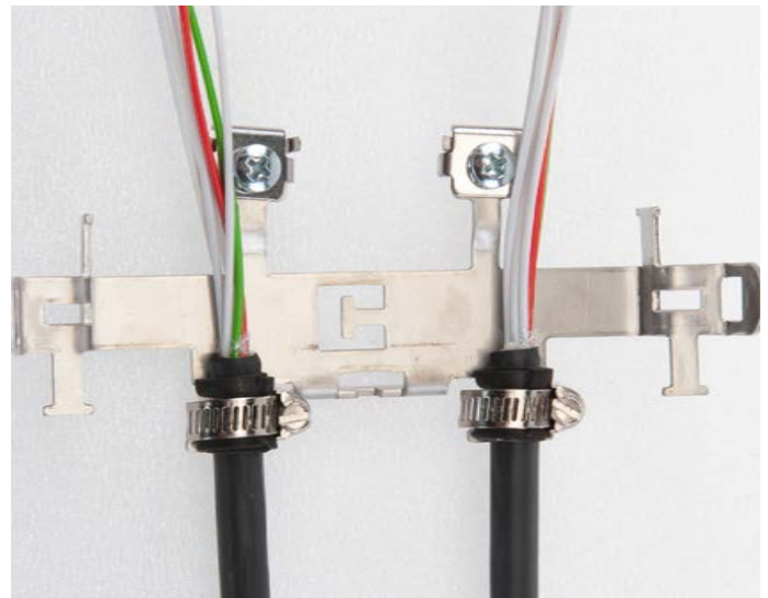
6.2.5 Secure cable jacket with hose clamps, position head of hose clamp at the inside of the bracket.
