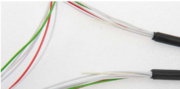
6.2.3 Cut the strength members at 40 mm/1.57 inches from jacket end.
