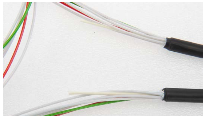
6.1.3 Cut the strength members at 60 mm/2.36 inches from jacket end.
