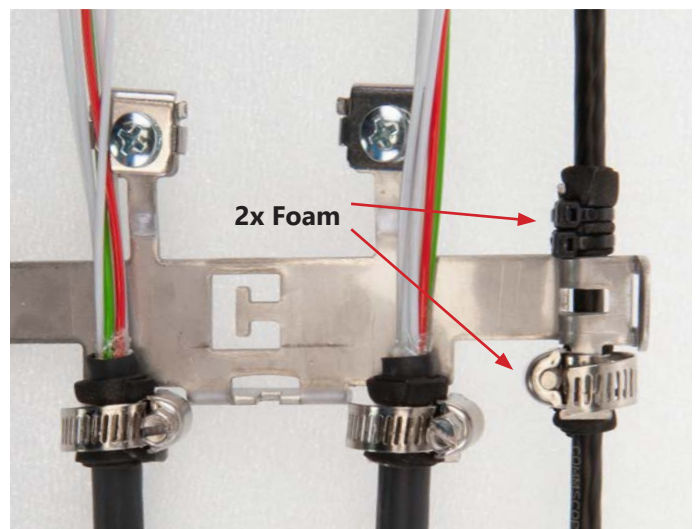
6.2.6 Note that the strain relief of the branch cable does not include the strength member. Apply foam on each side of the bracket as shown and secure with hose clamp and tie-wraps or with 2 hose clamps.
