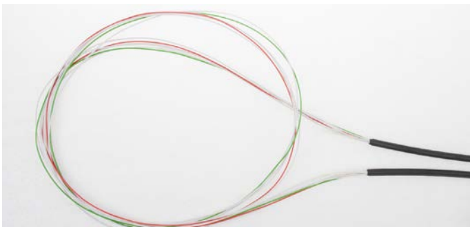
6.2.2 Make a window cut of 2.2 m/86.6 inches. When uncut fibers need to be stored, make sure that the twisting point (SZ) is in the middle.
