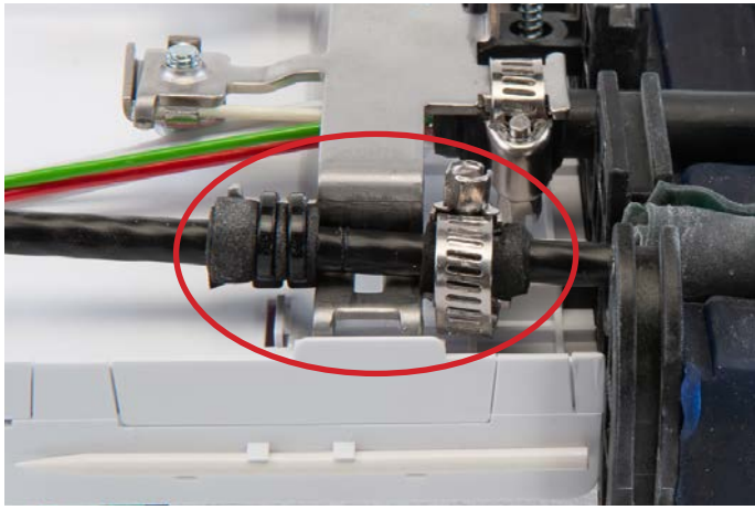
6.2.7 Install the assembly to the organizer (snap fit at both sides).
