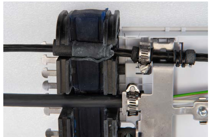
7.2.2 Bracket 2 installed.
