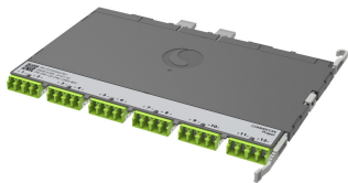
Propel ULL Multimode OM5 MPO-12 Distribution Module, 12 duplex LC to 2X12f MPO/UPC non-pinned, Method B Enhanced
