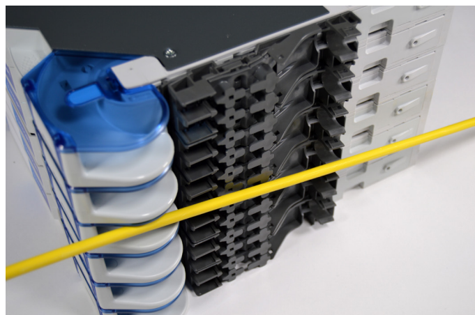
5.5.1. A high fiber count loose tube cable can be routed with a maximum of 6 FACT elements. Use the CTU bracket mounted in the middle of the row for mounting the cable. Route and divide the loose tubes via the shortest and most bendless way to the different CTU elements.
