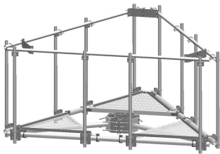
Upper Support Rail Kit for co-location platforms, 12 ft face with XA-U Universal Cross-over
