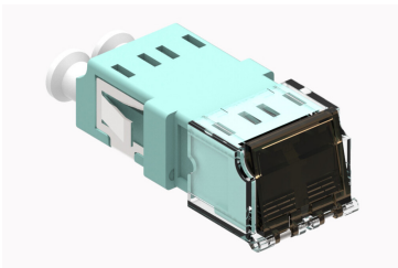
LazrSPEED® LC Duplex Low Profile Shuttered Adapter, Aqua, Single Pack
