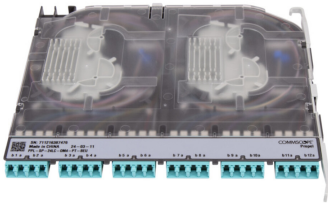
Propel Multimode Splice Cassette, 24LC with internal shutters, OM4 single fiber pigtails, Method B Enhanced ULL
