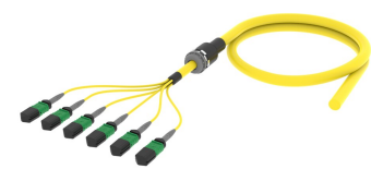
Singlemode MPO8 APC (pinned) to Unconnectorized Fiber Trunk Cable Assembly, 48-Fiber, Armored Indoor Plenum
