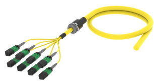
Singlemode MPO8 APC (pinned) to Unconnectorized Fiber Trunk Cable Assembly, 64-Fiber, Armored Indoor Plenum
